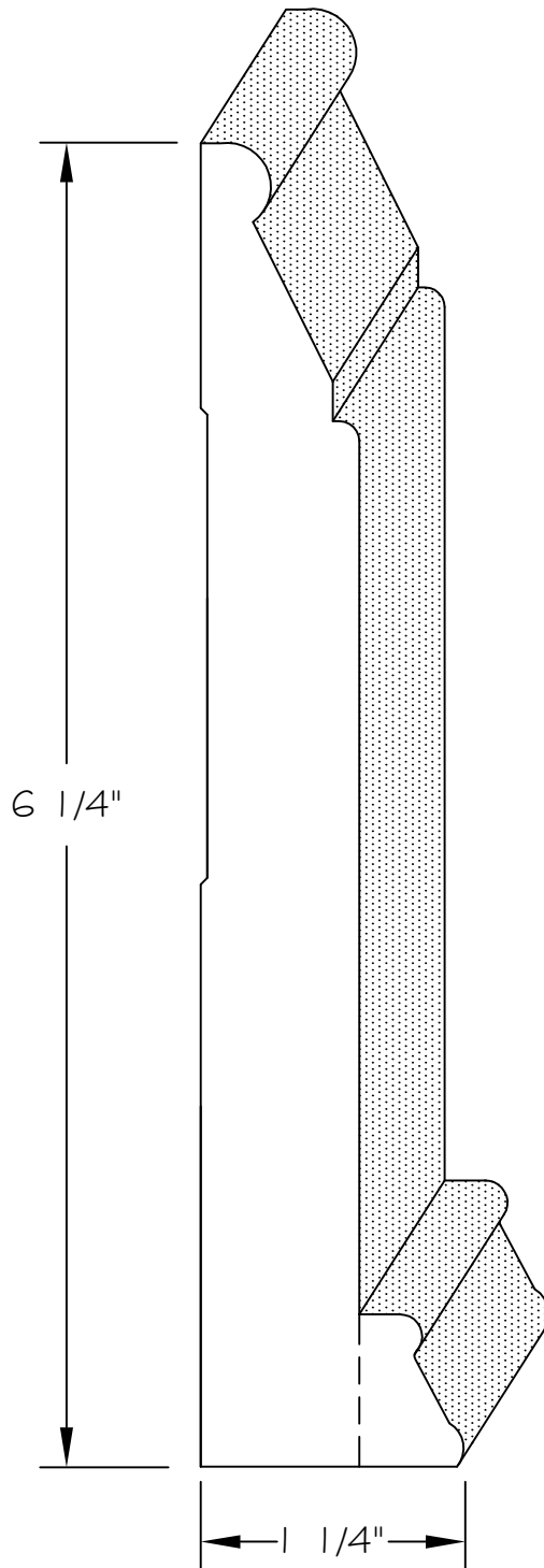
BB-107 - Baseboard /w Base Shoe 6-1/4"x 3/4" **
