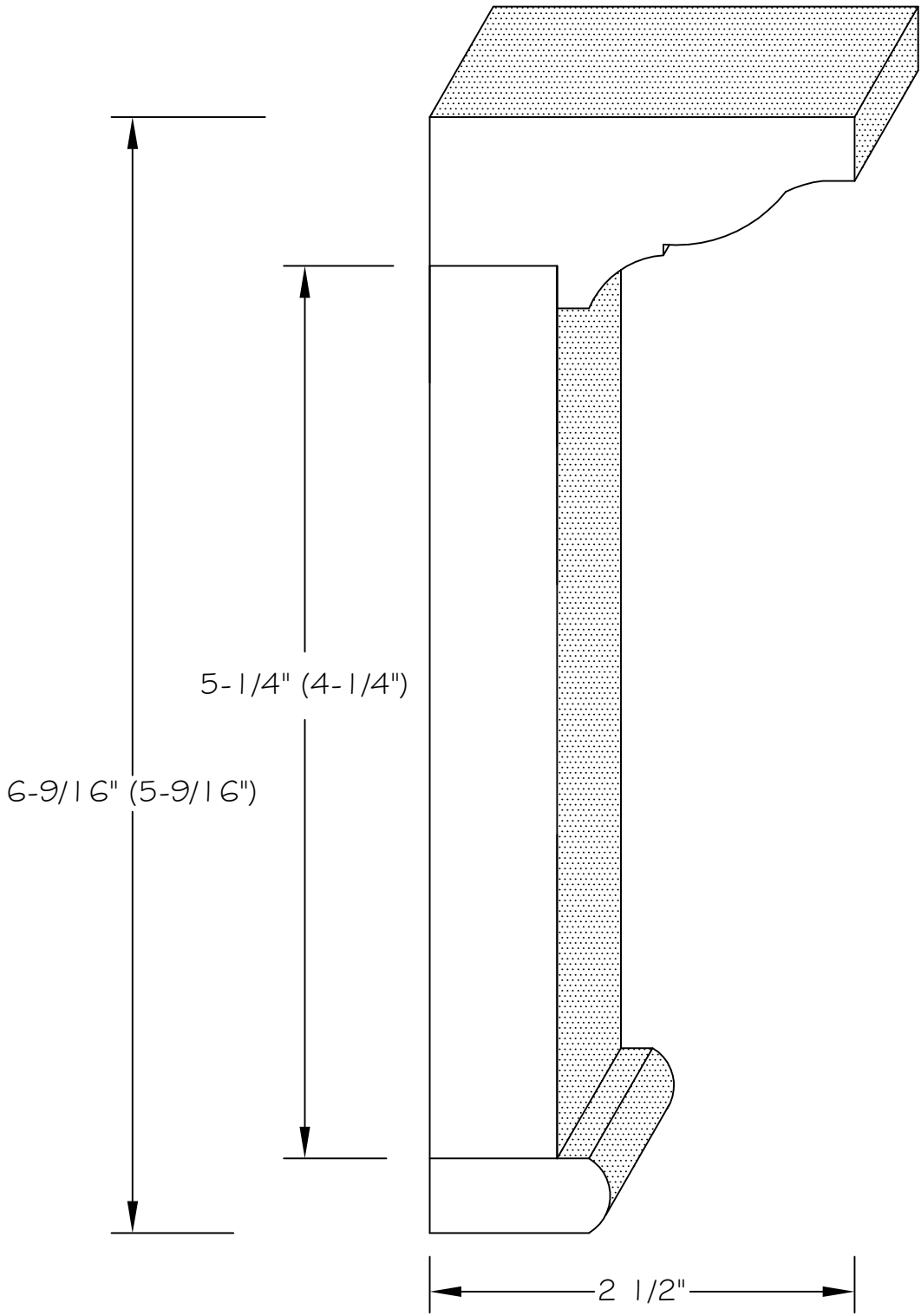
HD-1008 - 3-pce Boston Header 5\frac{1}{4} " (or 4\frac{1}{4} ") x 2\frac{1}{2} "
