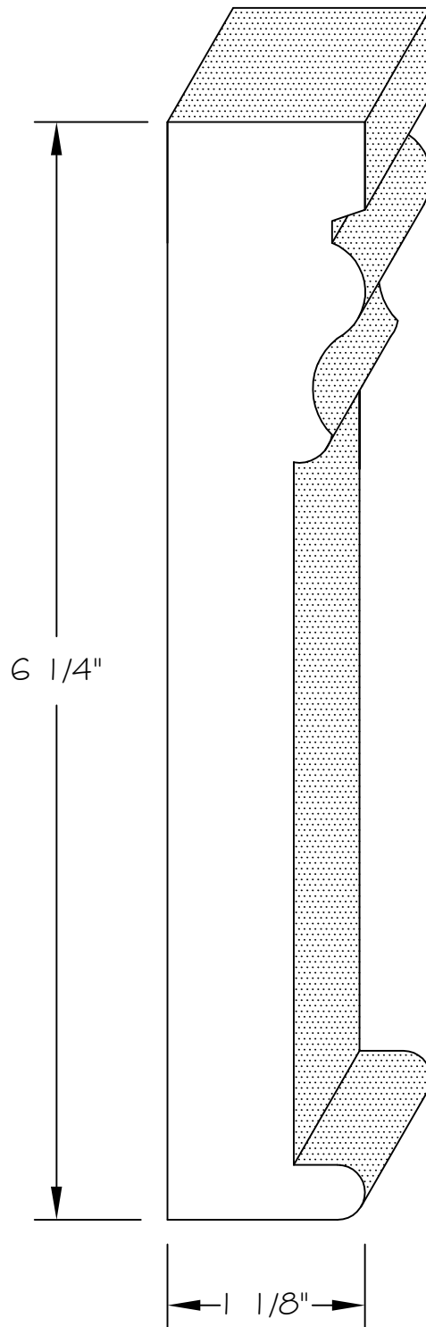
HD-1009 - 1-pce Boston Header 6-1/4" x 1-1/8"
