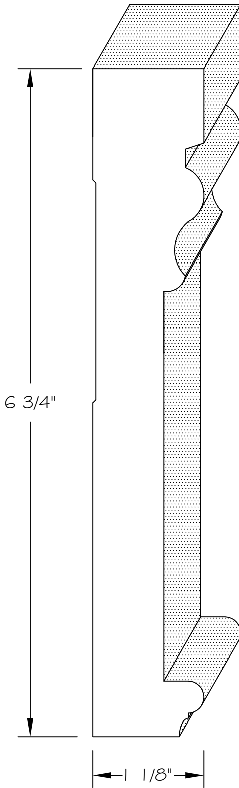
HD-1010 - 1-pce Boston Header 6-3/4" x 1-1/8"
