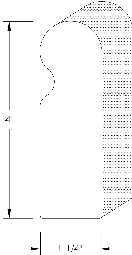
HR-805 - Handrail 1 - 1/4" x 4"
