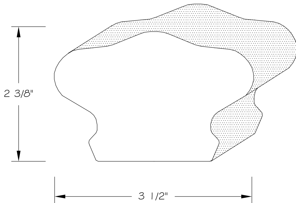
HR-807 - Handrail 3-1/2" x 2-3/8"
