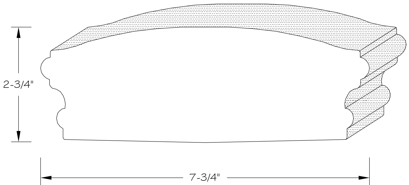
HR-808 - Handrail 7-3/4" x 2-3/4"
