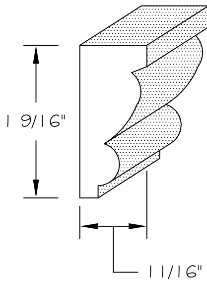
PM-404 - Panel Moulding 1 \frac{9}{16} " x 1 \frac{1}{16} "
